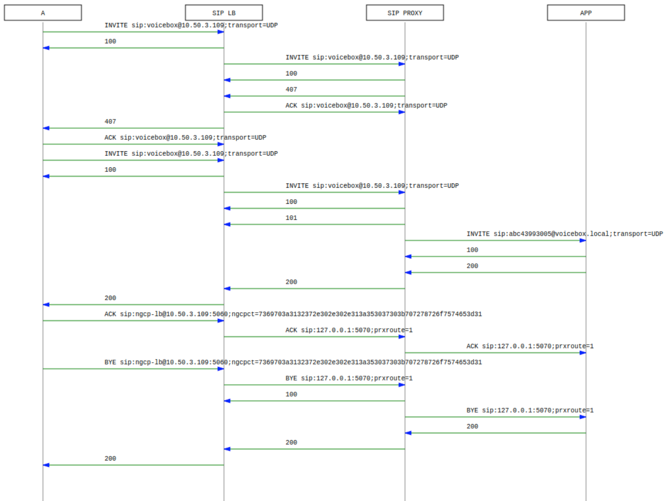
Figure 75. Voicebox Call-Flow
