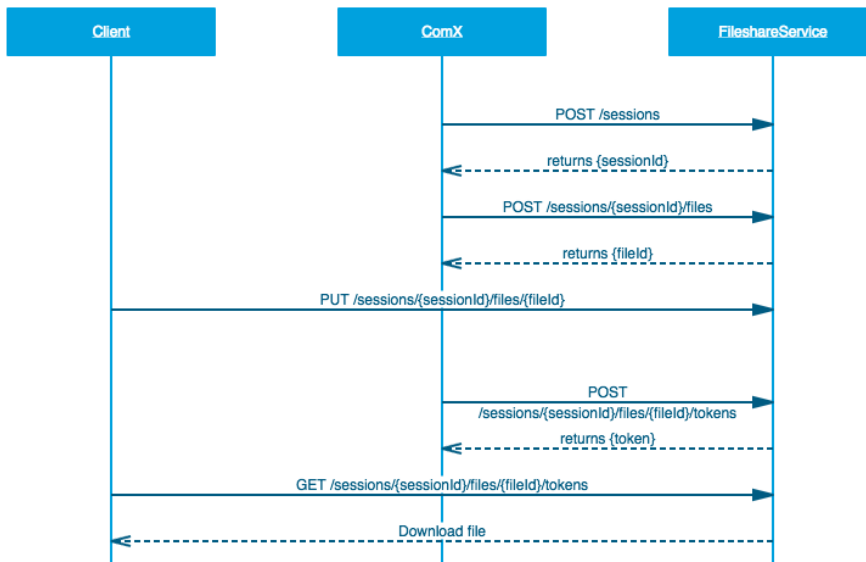
Figure 181. Sequence Simple
