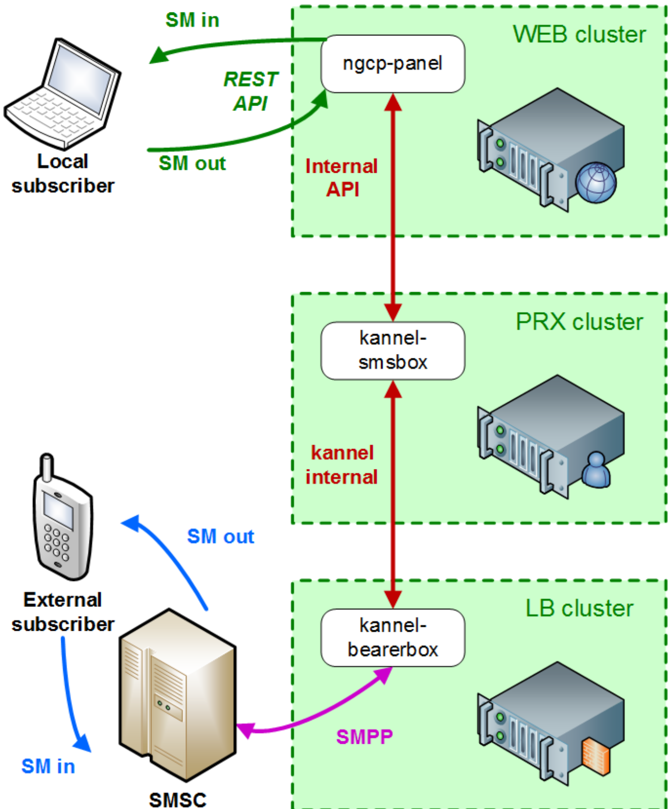
Figure 179. SMS Interaction
