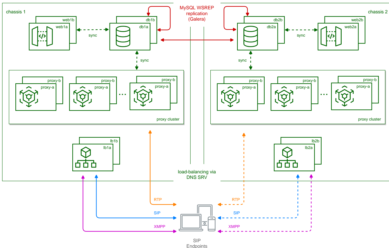
Figure 12. Scaling beyond one chassis
