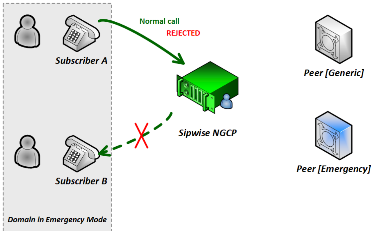
Figure 86. Call-flow in Emergency Mode 1. (Std to Std)
