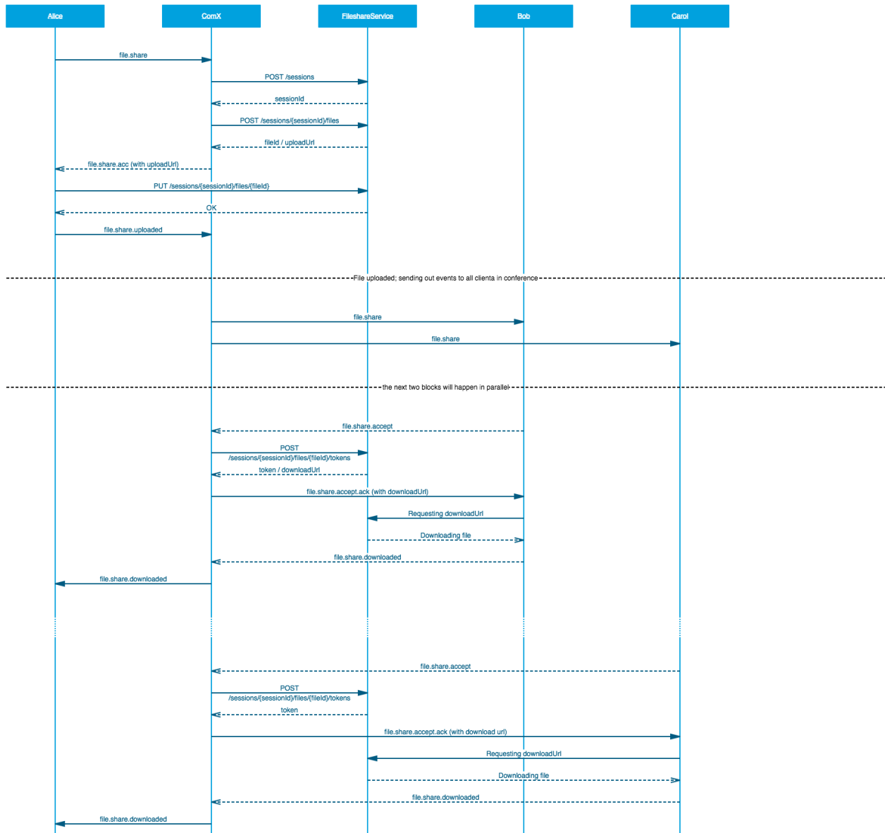
Figure 182. Sequence Detailed
