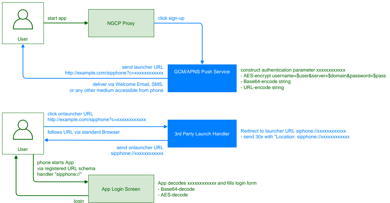
Figure 164. Provisioning Push Workflow
