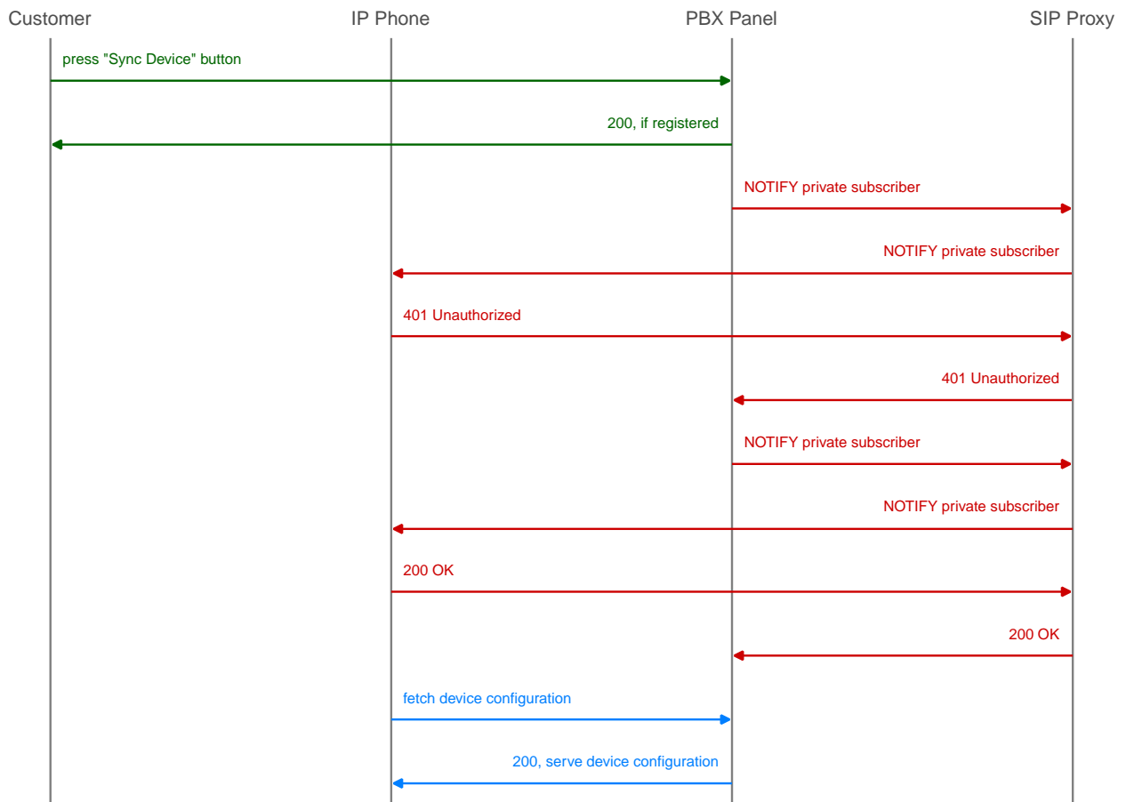
Figure 151. Resync a registered PBX device
