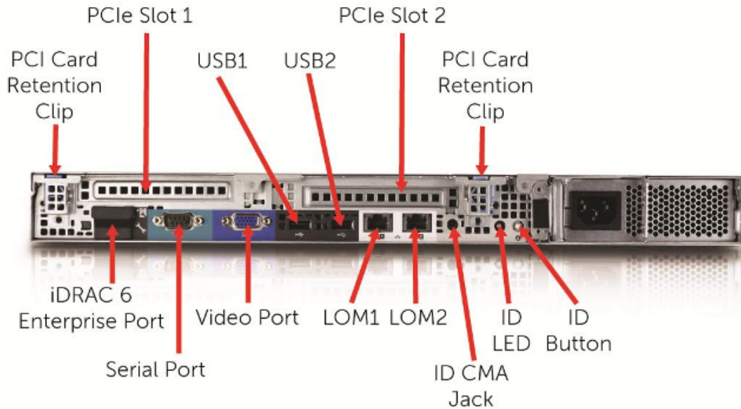
Figure 18. Dell R310 Rear View
