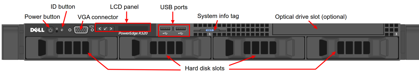
Figure 16. Dell R320 Front View
