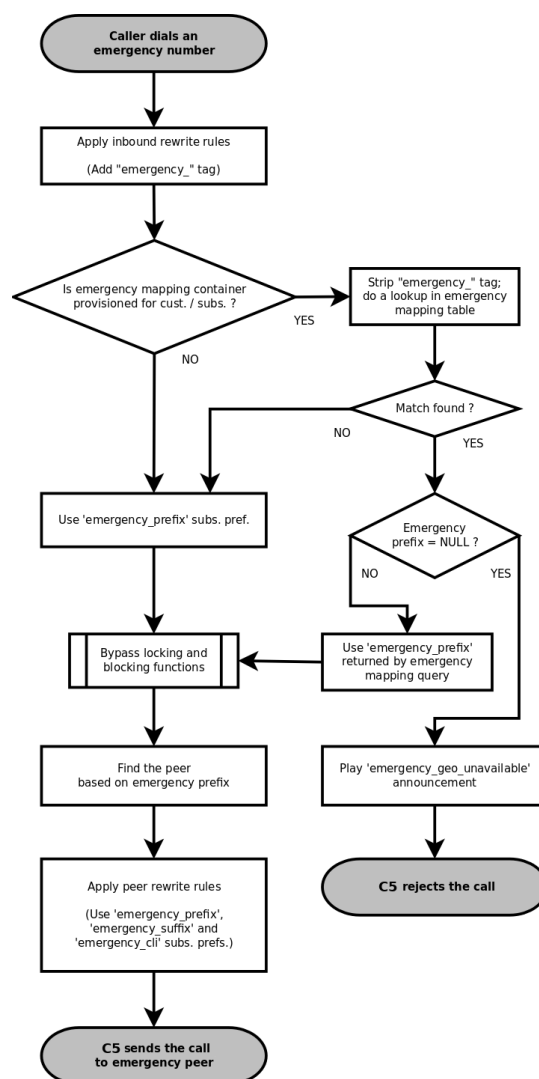
Figure 80. Emergency Call Handling with Mapping
