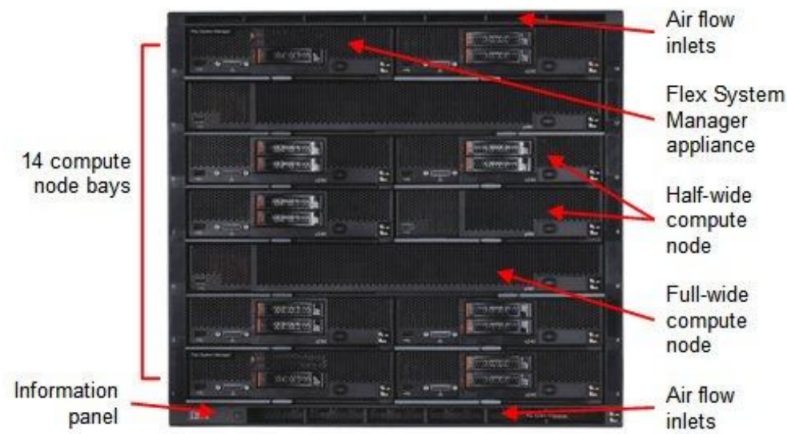
Figure 9. Chassis front view
