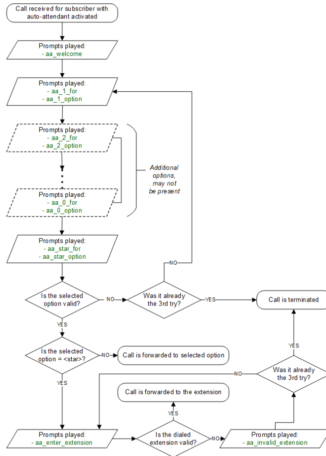
Figure 145. Flowchart of Auto-Attendant
