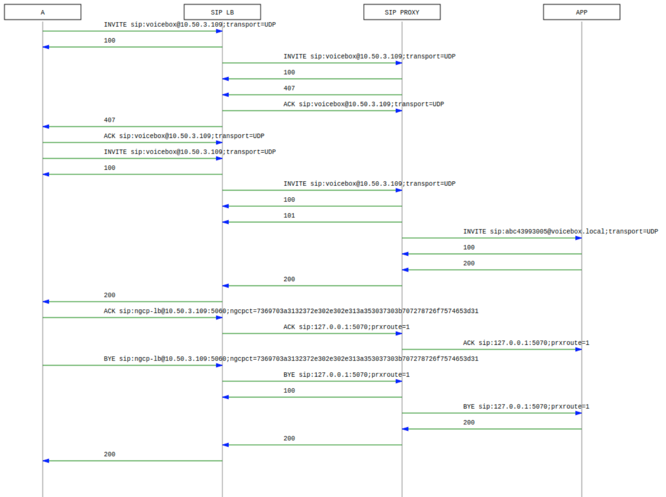
Figure 191: Voicebox Call-Flow
