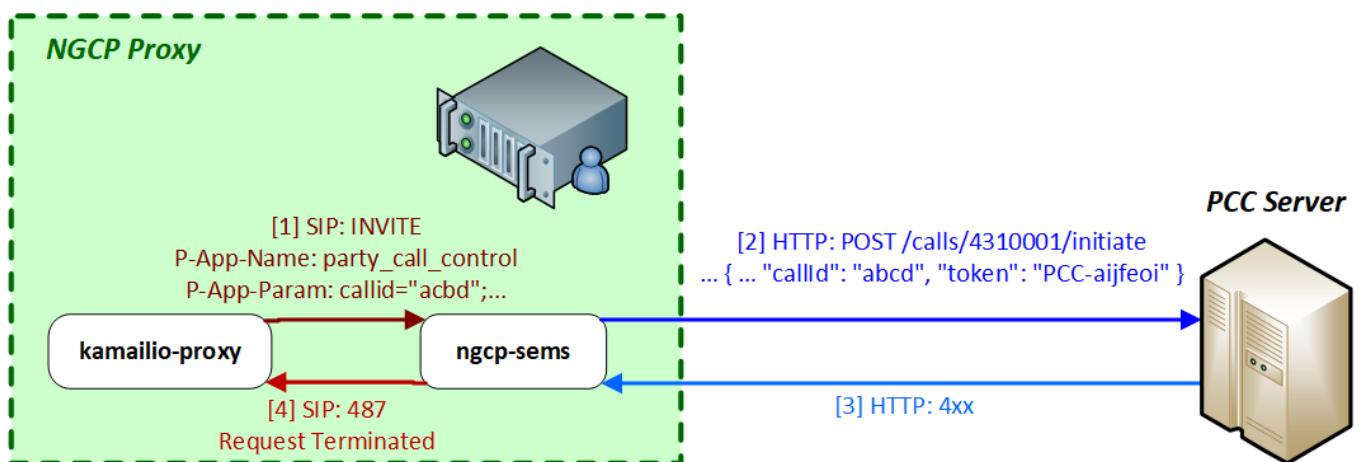
Figure 180: Call Initiation Error with PCC
