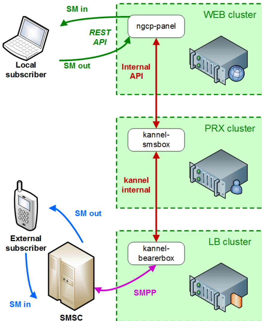
Figure 82: SMS Interaction
