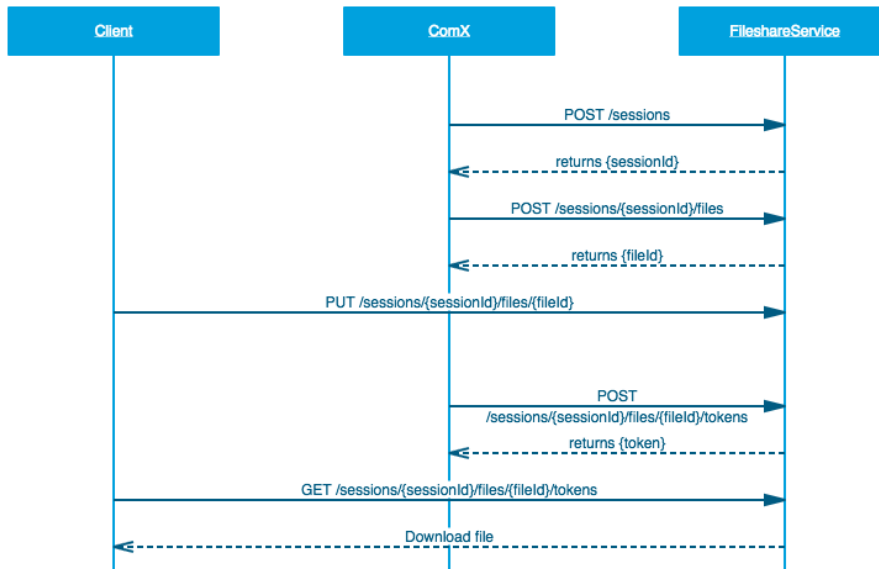
Figure 196: Sequence Simple
