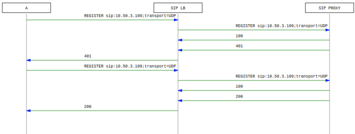
Figure 189: Registration Call-Flow
