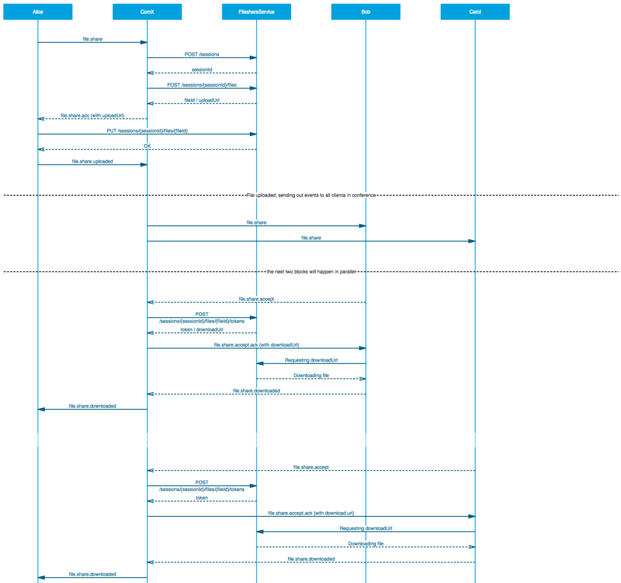
Figure 197: Sequence Detailed
