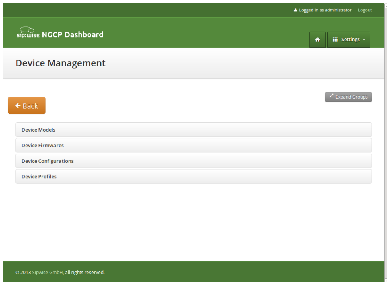
Figure 165: Device Management
