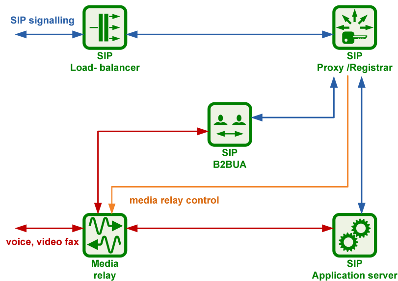
Figure 2: SIP and Media Relay Components
