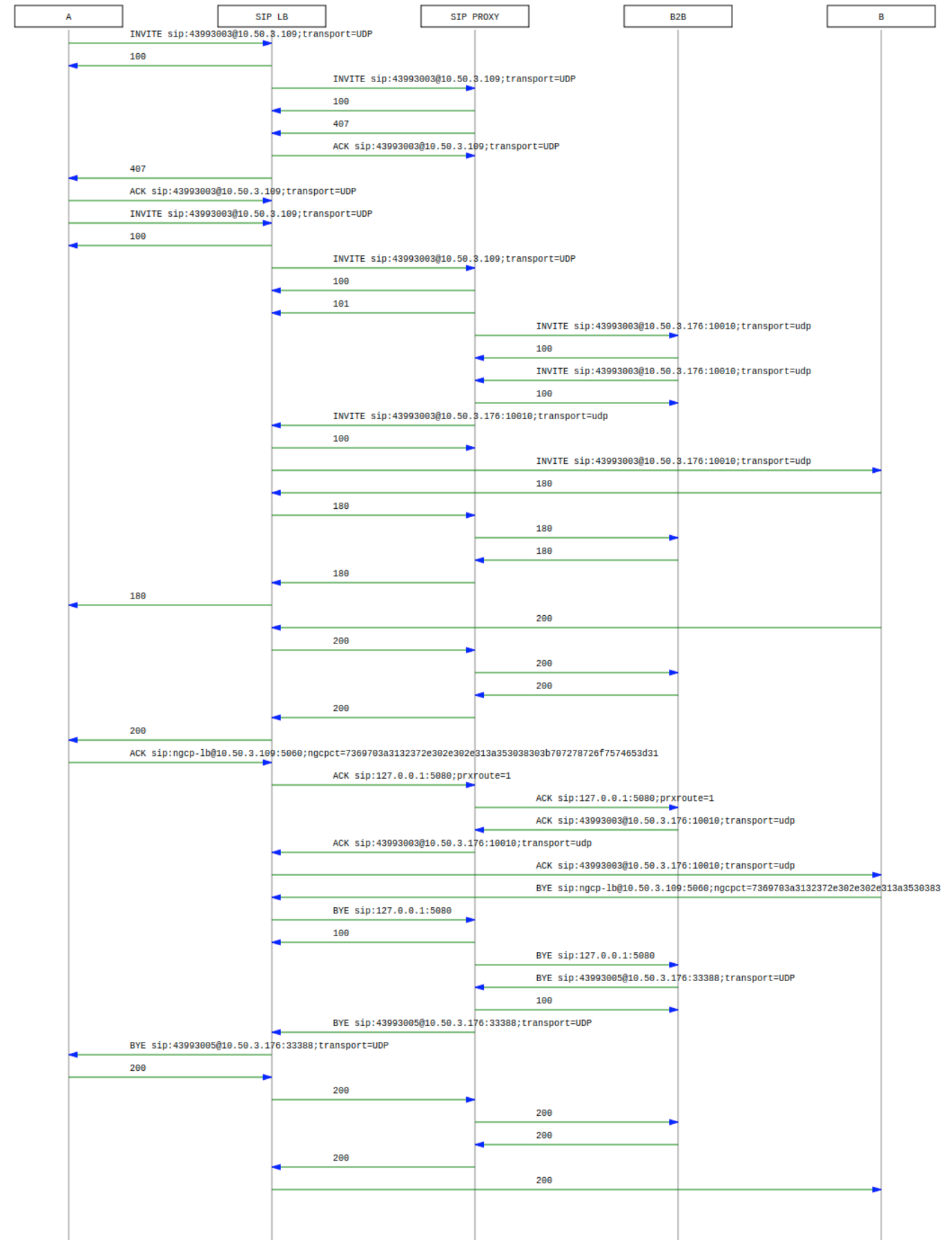
Figure 76: Basic Call Call-Flow
