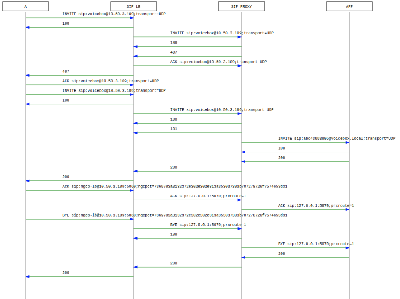
Figure 77: Voicebox Call-Flow
