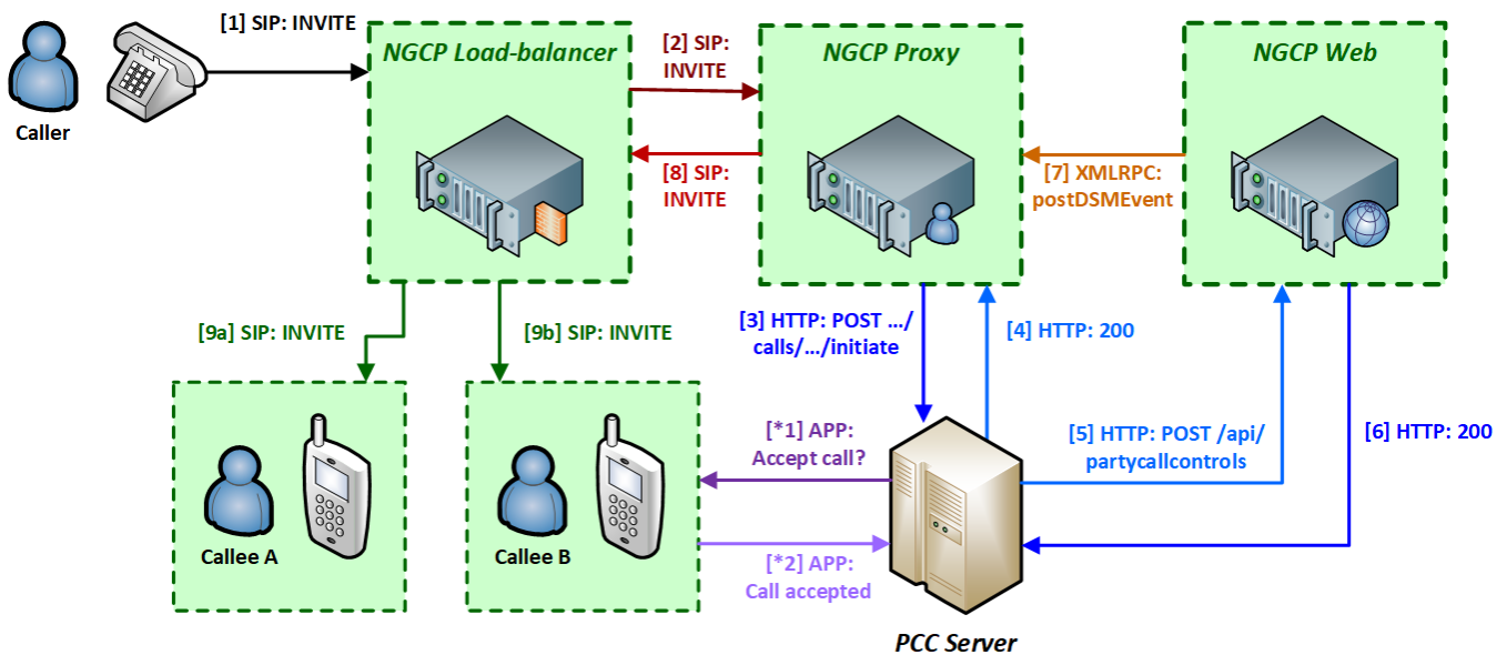
Figure 166: Overview of Party Call Control
