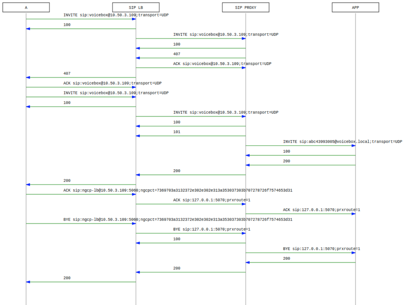
Figure 179: Voicebox Call-Flow
