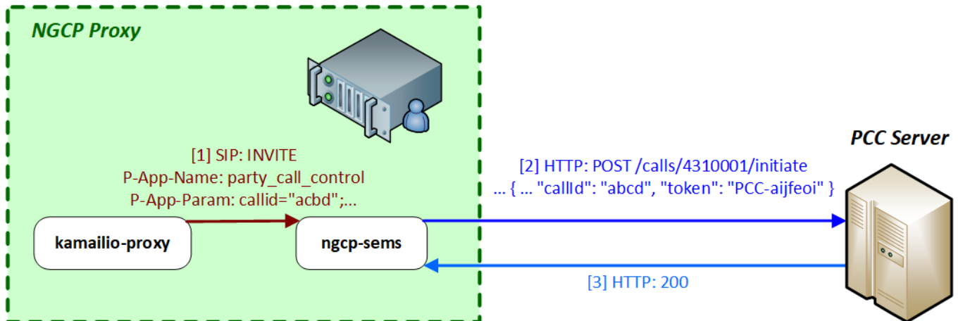
Figure 167: Successful Call Initiation with PCC
