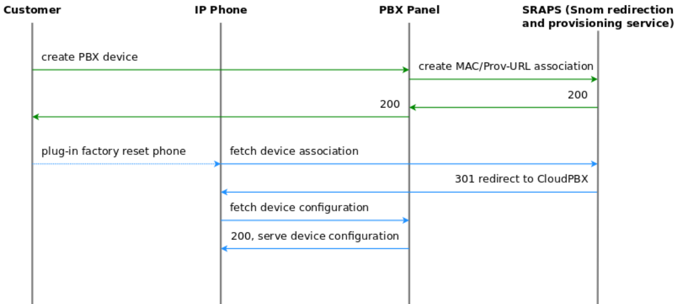
Figure 158: Initially bootstrap a SNOM phone
