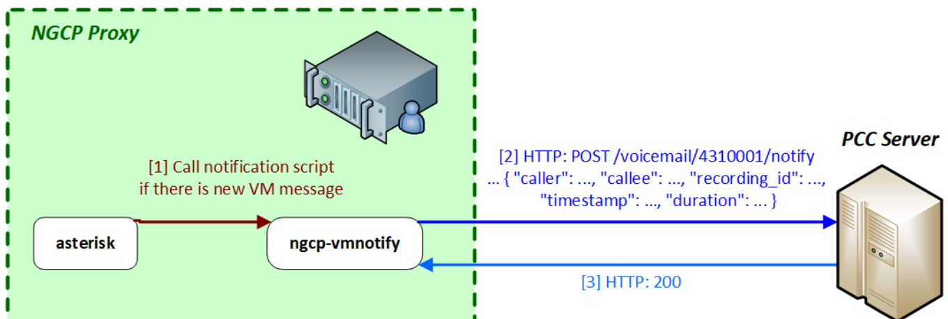
Figure 172: Voicemail Notification with PCC
