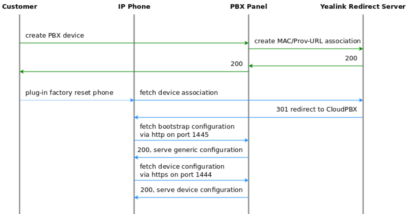
Figure 159: Initially bootstrap a Yealink phone
