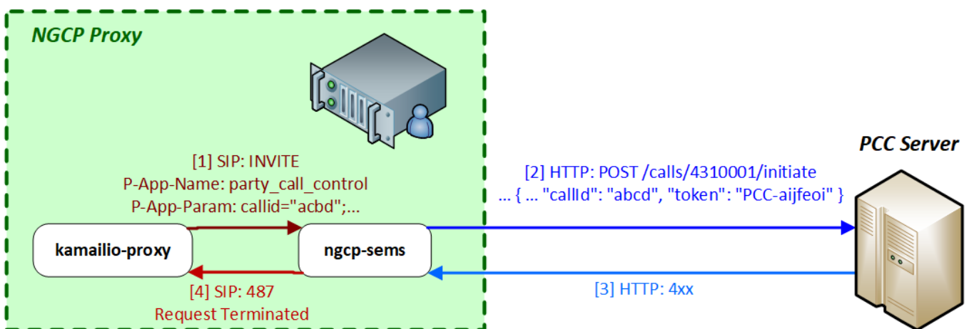
Figure 168: Call Initiation Error with PCC
