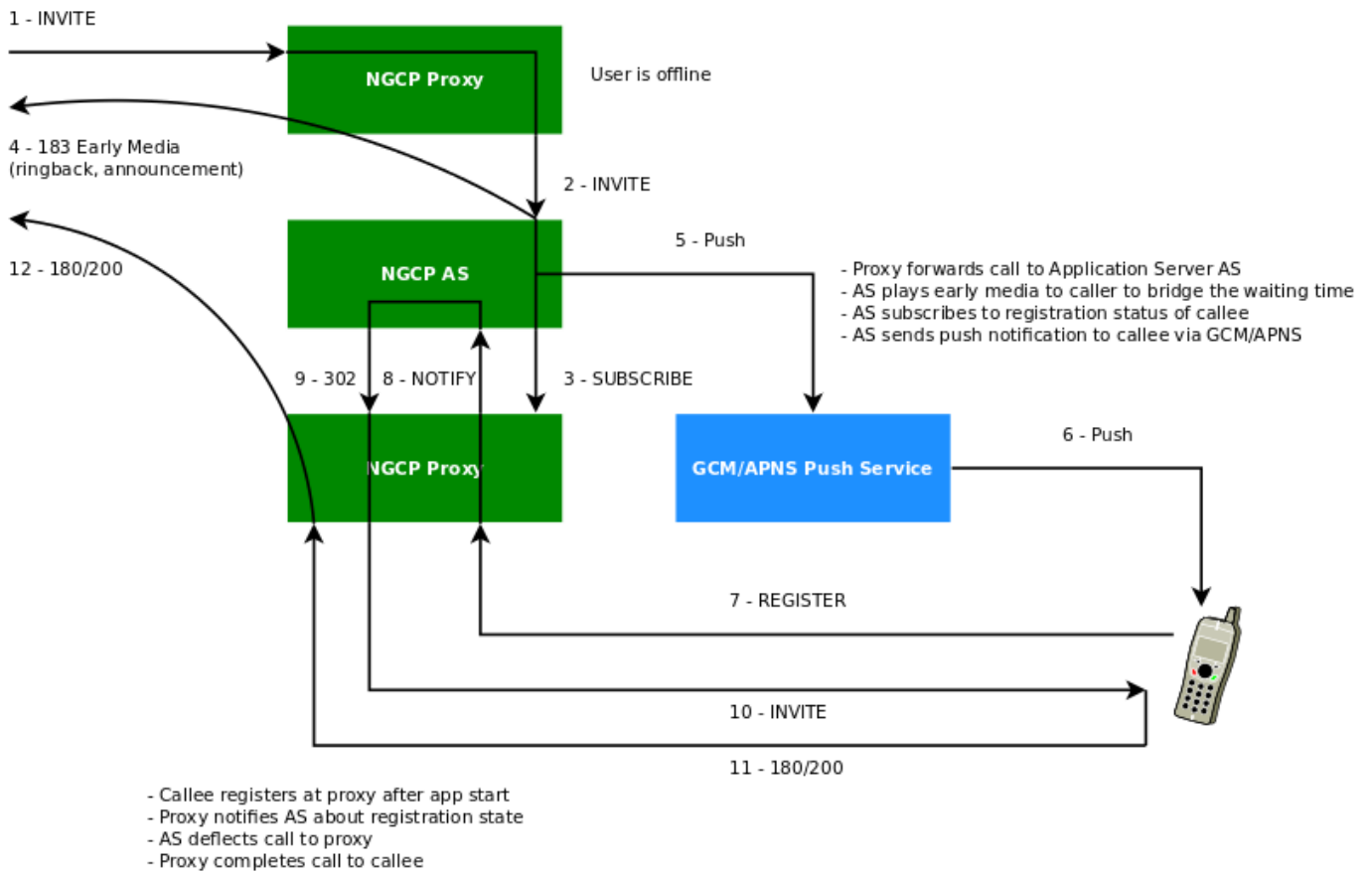
Figure 162: Mobile Push Workflow
