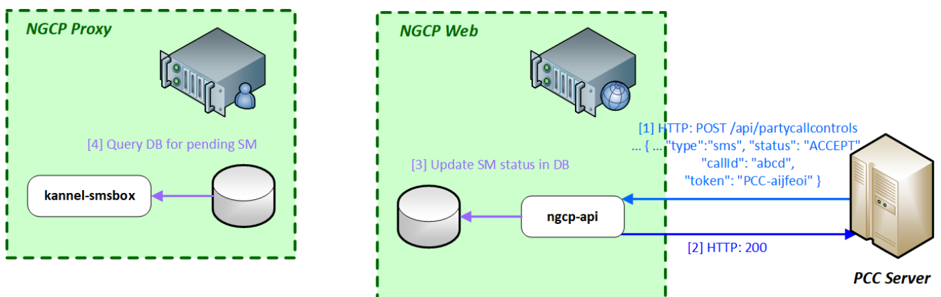
Figure 175: Short Message Accepted by PCC
