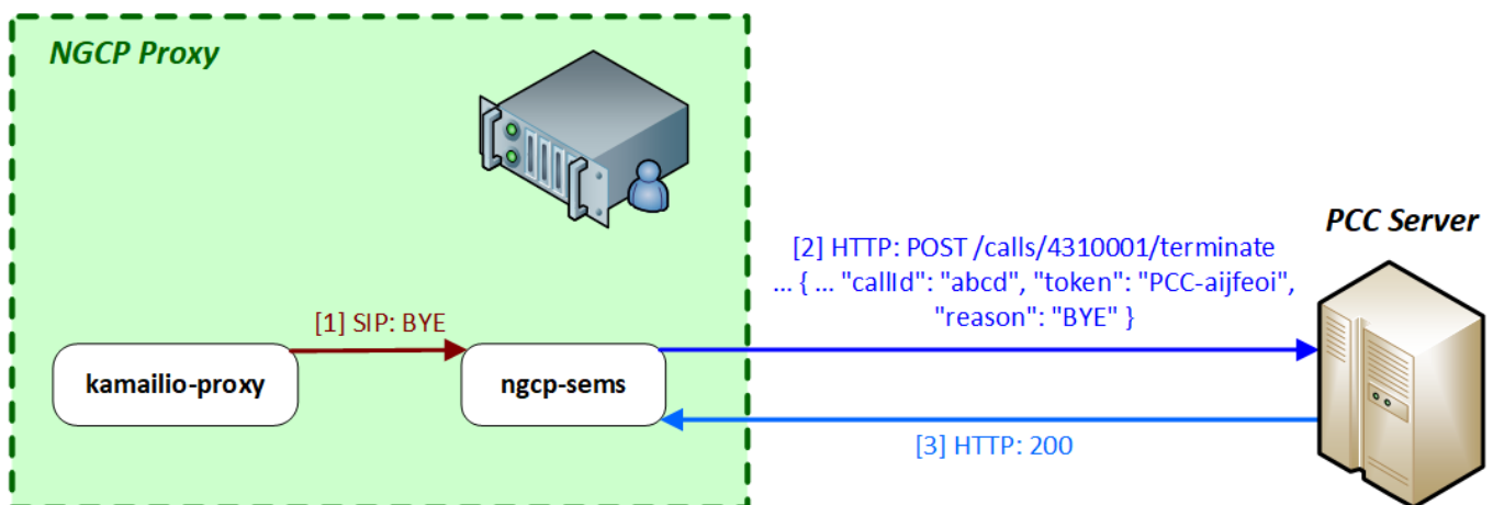
Figure 171: Call Termination with PCC
