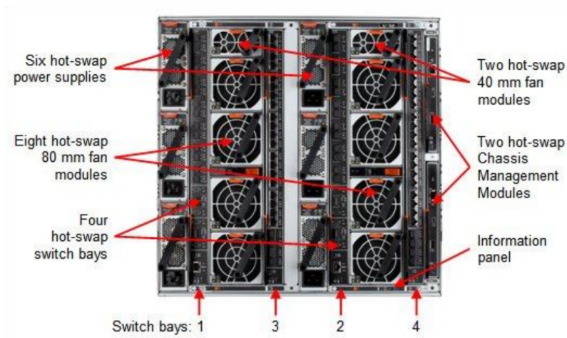
Figure 10: Chassis back view
