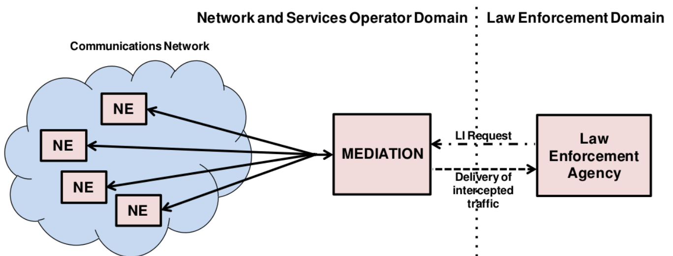
Figure 150: LI: High Level Overview
