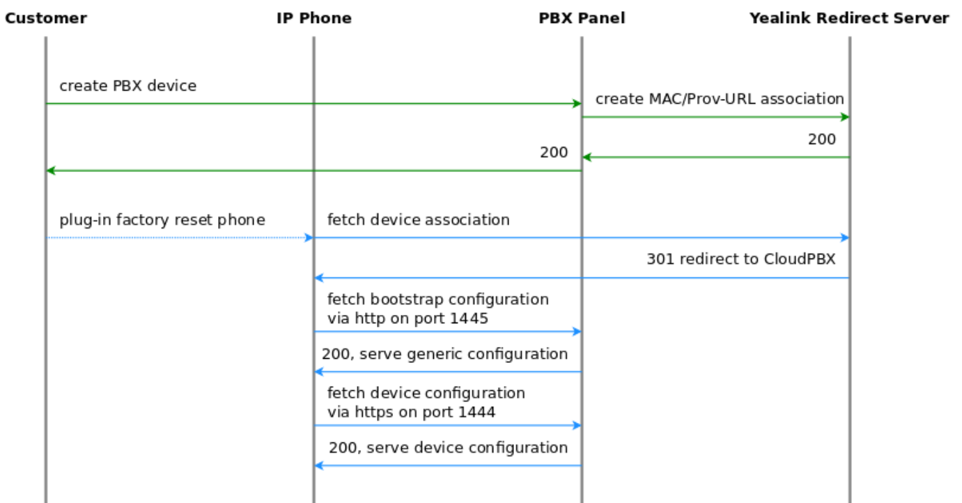
Figure 146: Initially bootstrap a Yealink phone
