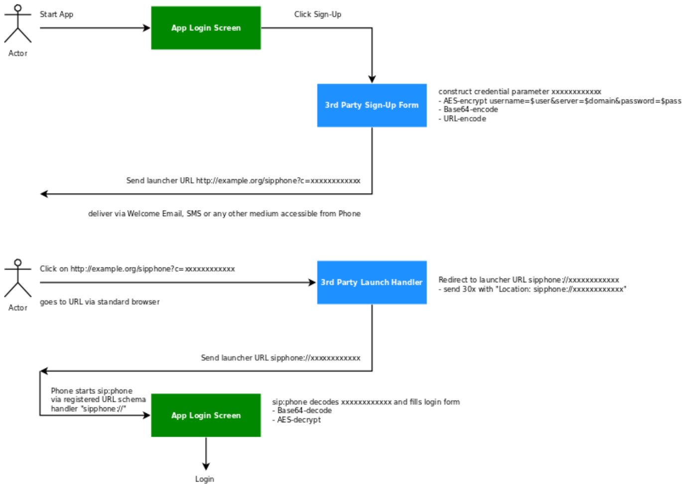
Figure 148: Provisioning Push Workflow
