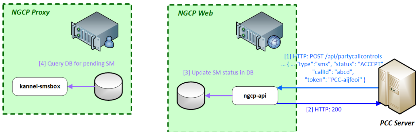
Figure 161: Short Message Accepted by PCC
