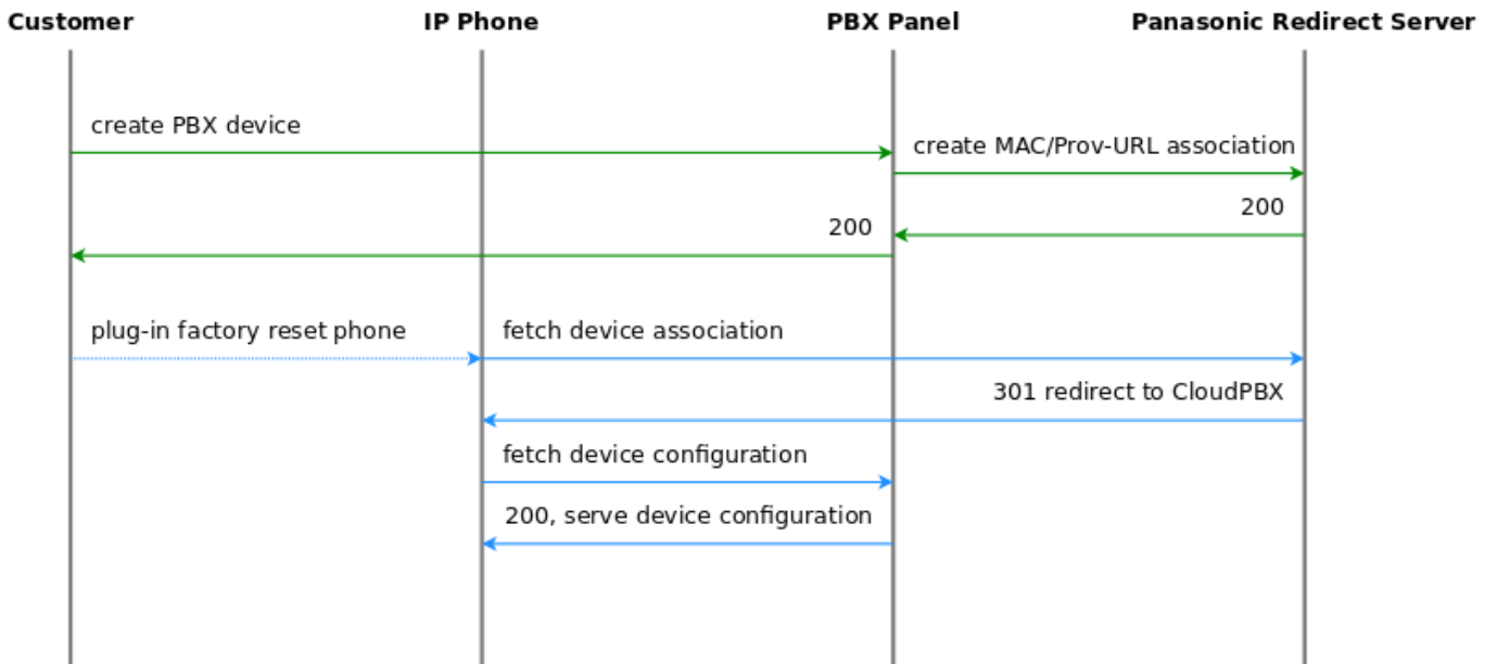
Figure 144: Initially bootstrap a Panasonic phone
