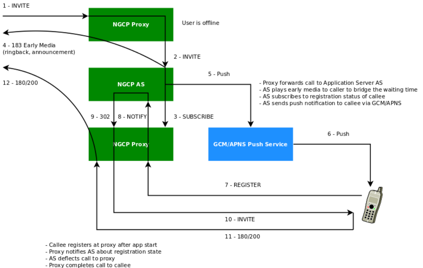
Figure 148: Mobile Push Workflow
