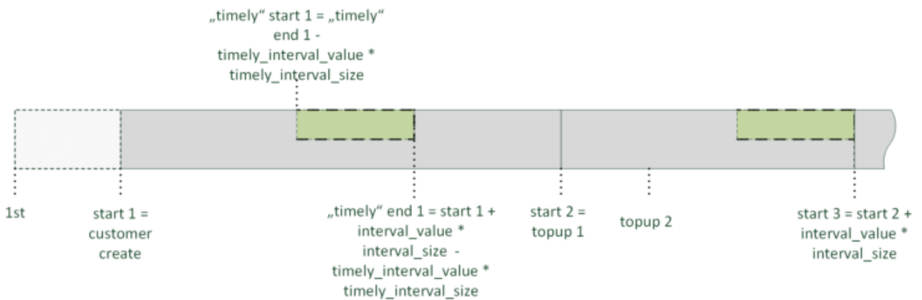
Figure 87: Interval Start Mode: topup_interval
