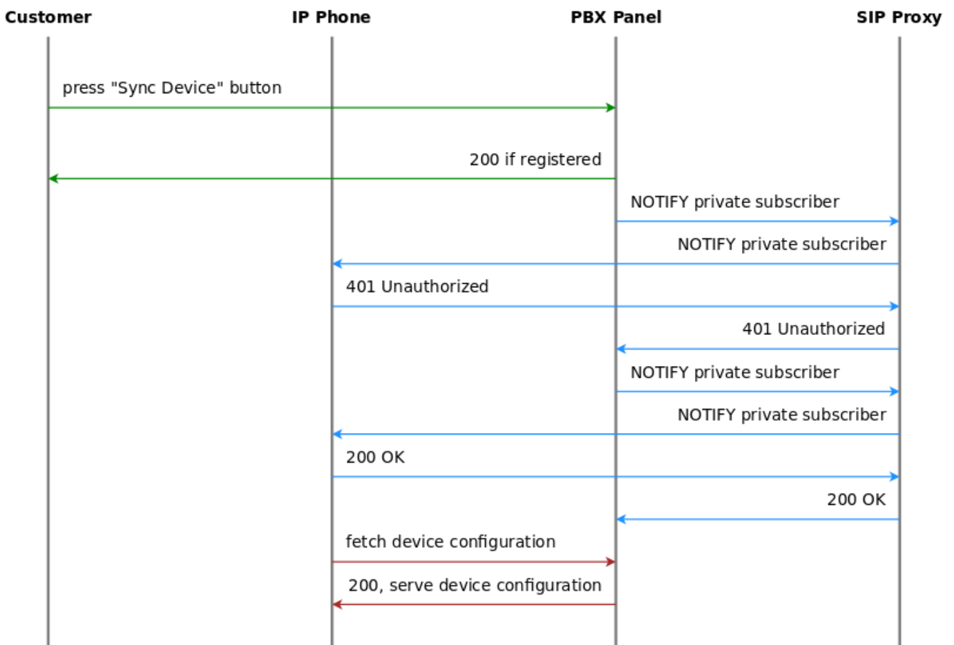
Figure 143: Resync a registered PBX device
