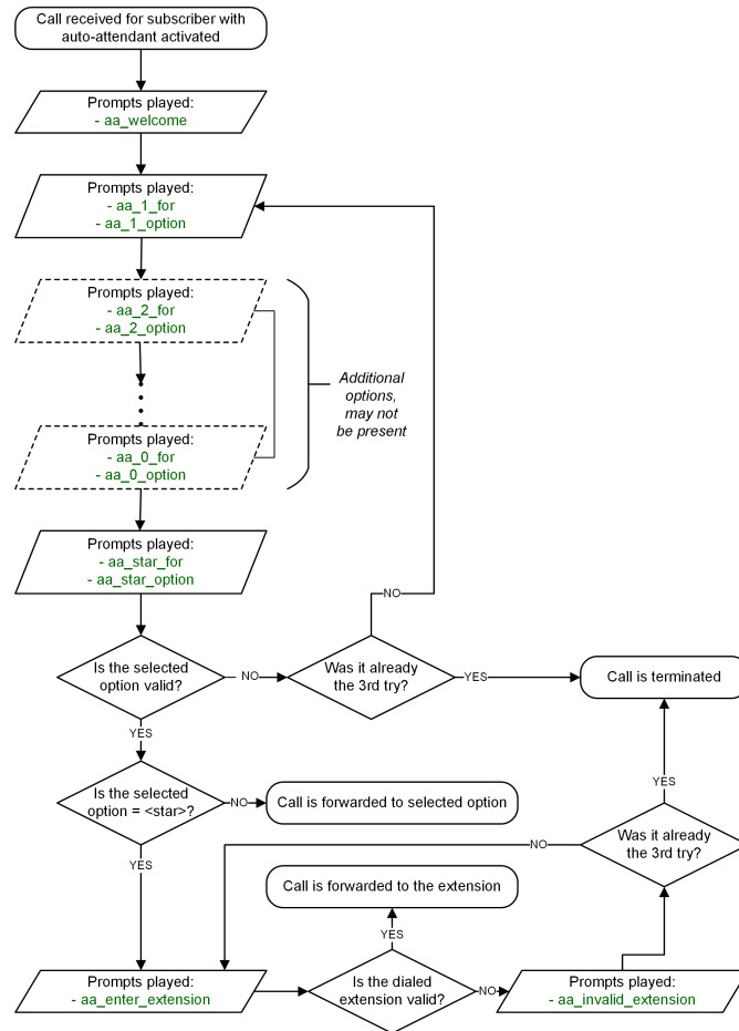
Figure 138: Flowchart of Auto-Attendant
