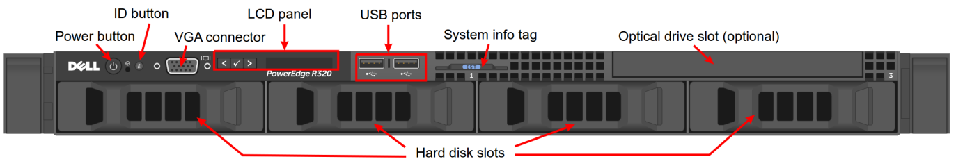
Figure 5: Dell R320 Front View
