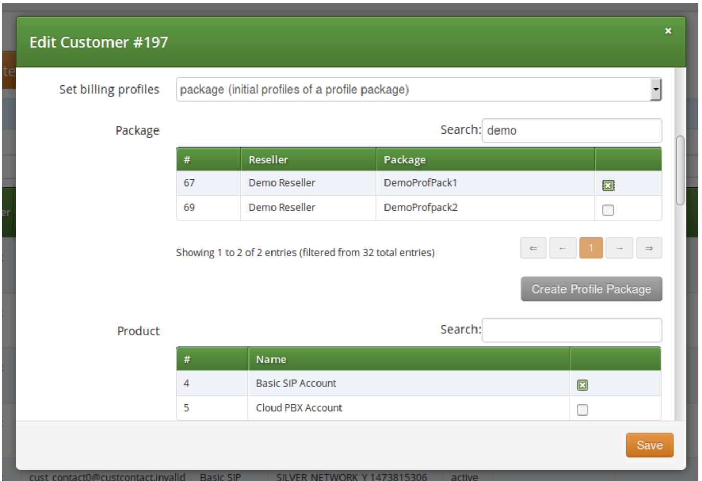
Figure 86: Assigning Profile Package to Customer
