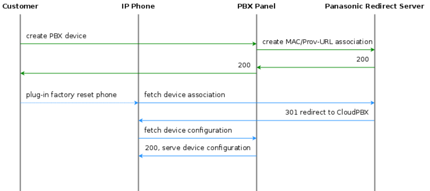
Figure 136: Initially bootstrap a Panasonic phone
