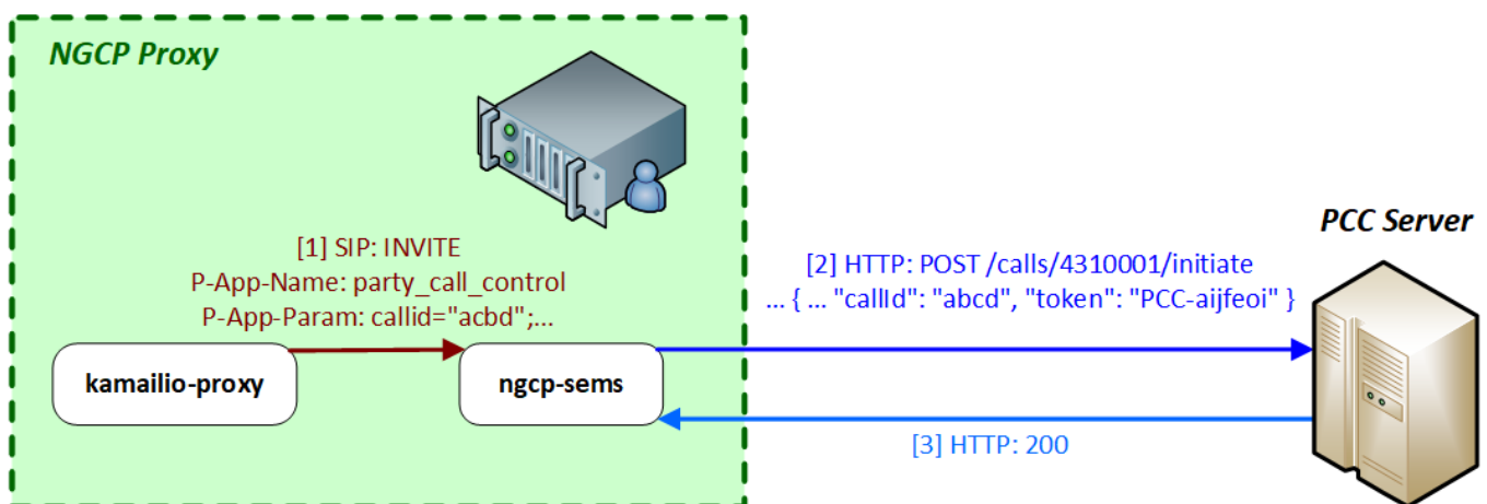
Figure 146: Successful Call Initiation with PCC
