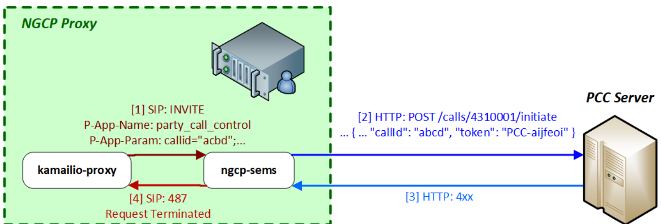
Figure 147: Call Initiation Error with PCC
