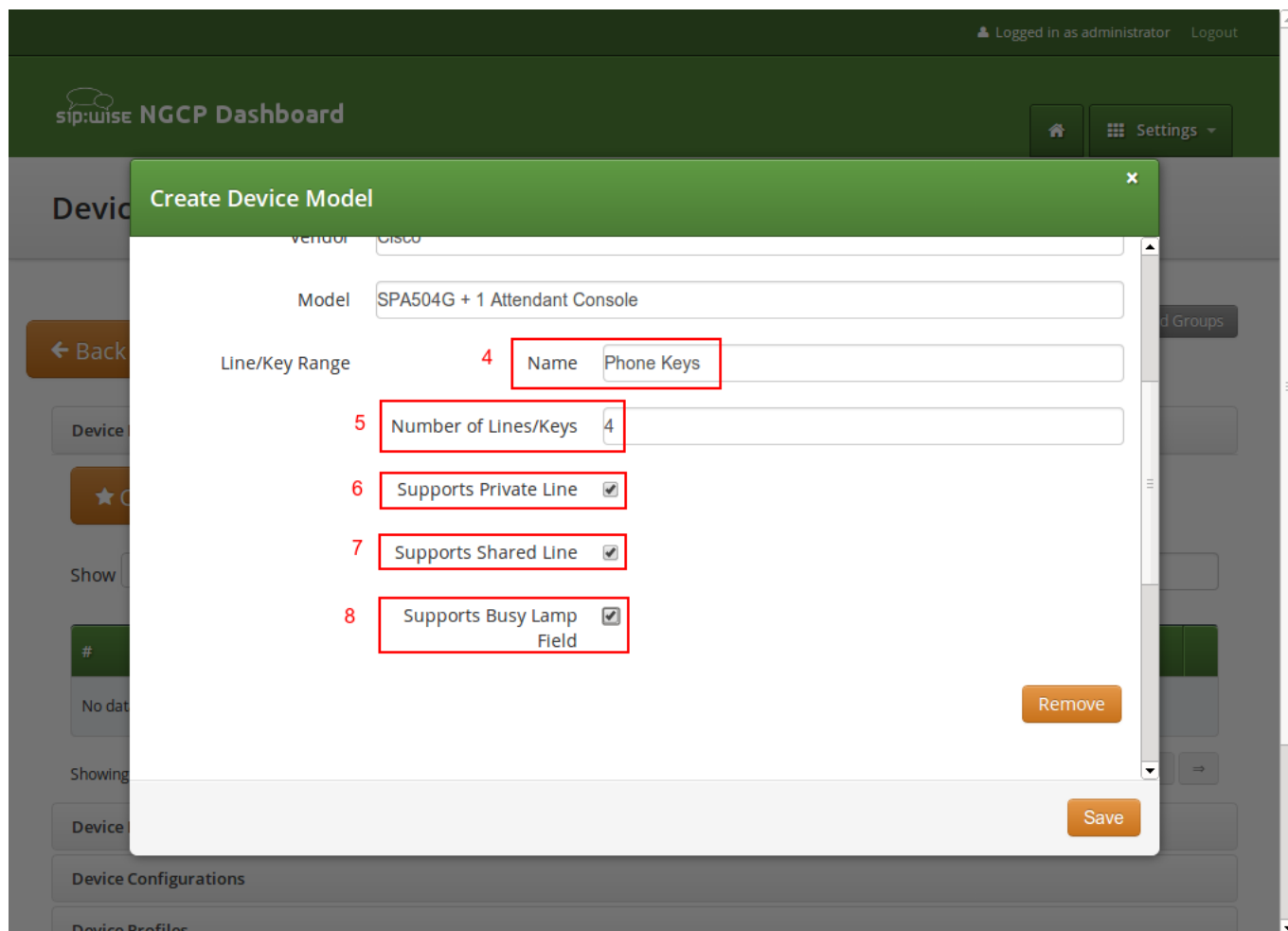
Figure 164: Create Device Model Part 2
