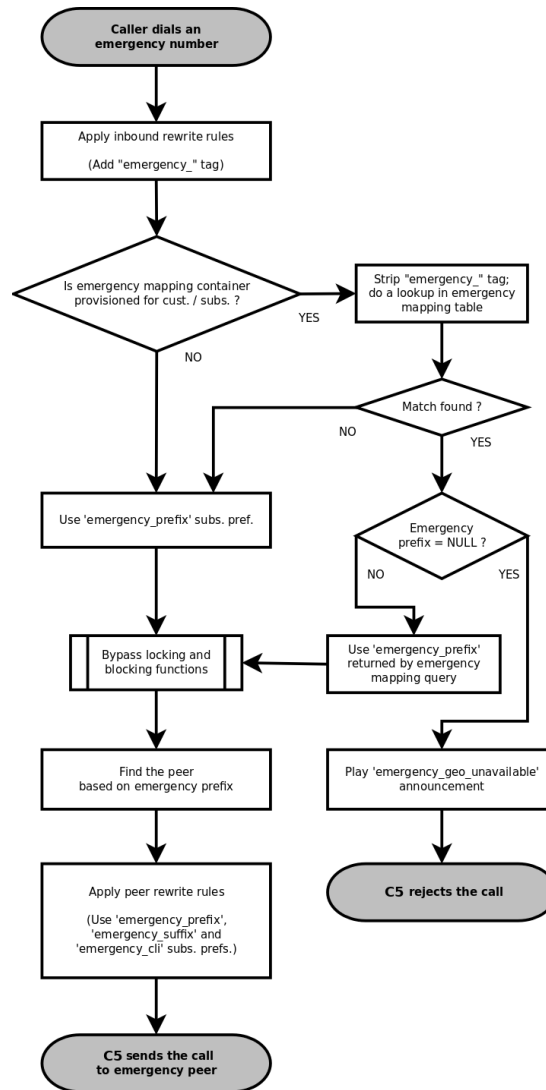
Figure 37: Emergency Call Handling with Mapping
