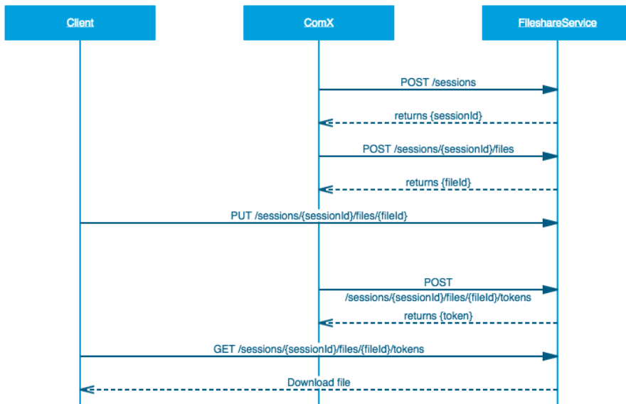
Figure 169: Sequence Simple
