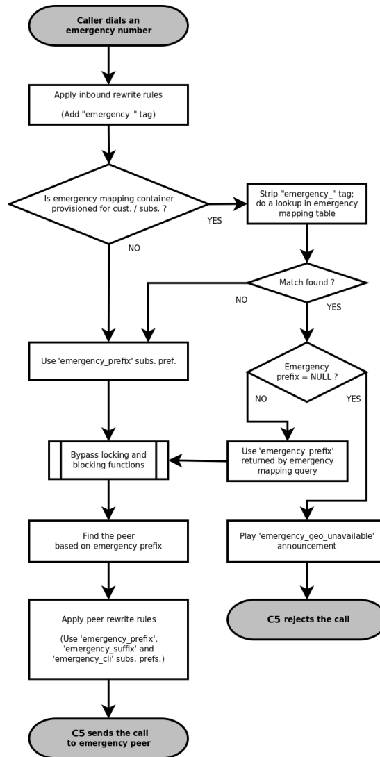
Figure 34: Emergency Call Handling with Mapping
