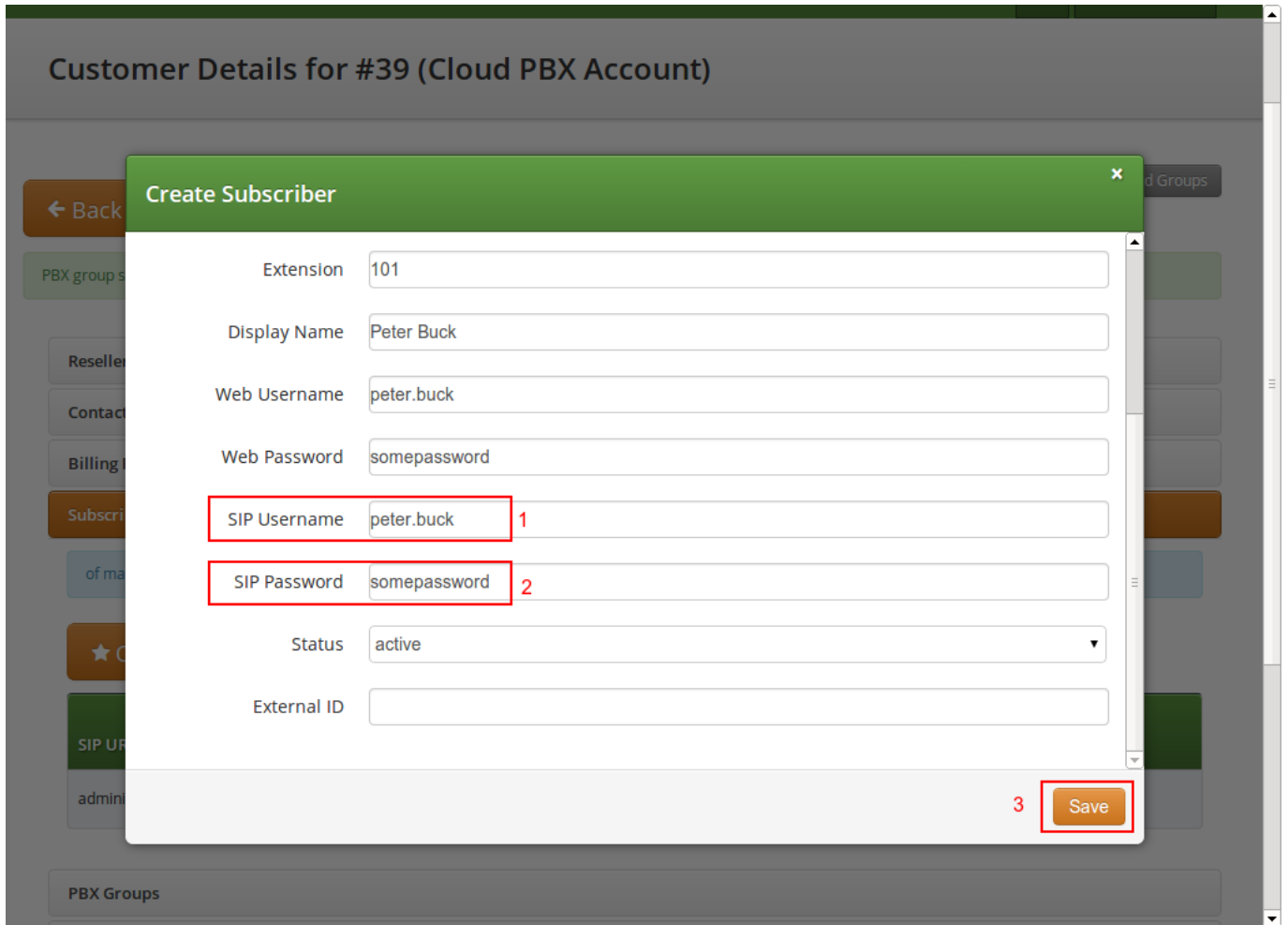
Figure 122: Finish PBX Subscriber Creation Part 2
