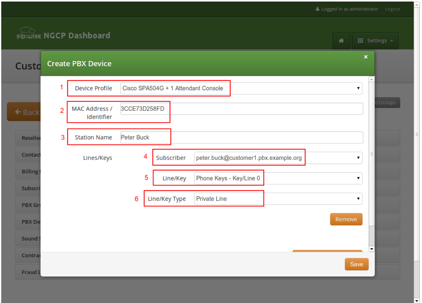
Figure 124: Configuring a PBX Device Part 1
