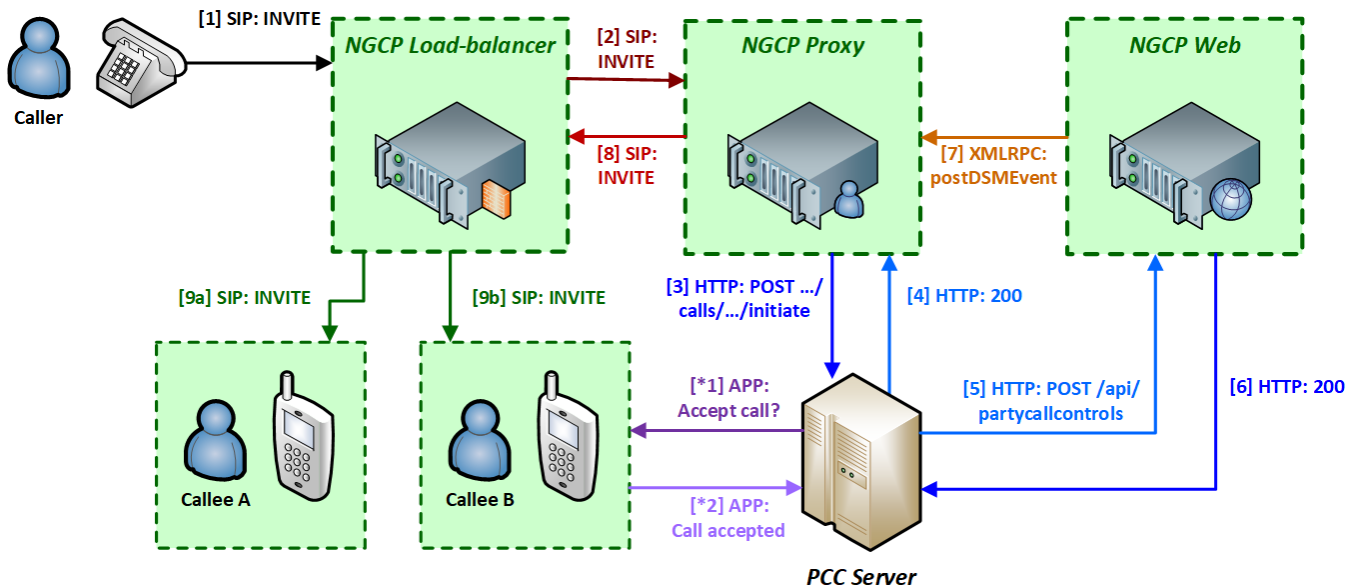
Figure 135: Overview of Party Call Control
