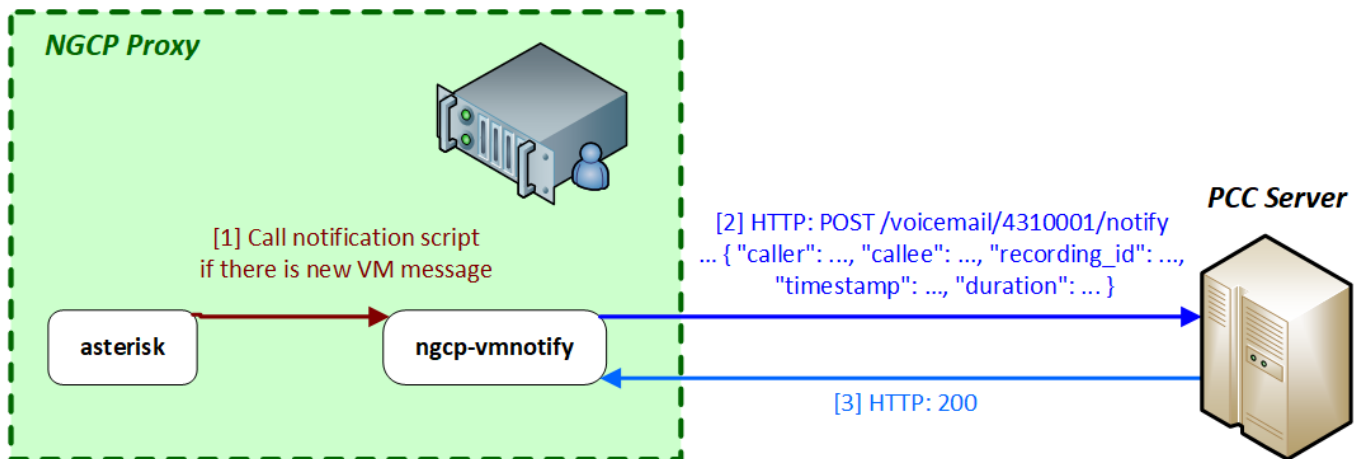
Figure 141: Voicemail Notification with PCC
