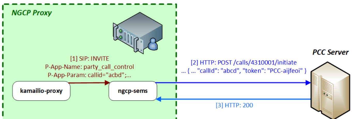
Figure 136: Successful Call Initiation with PCC
