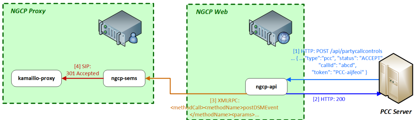
Figure 139: Call Accepted by PCC
