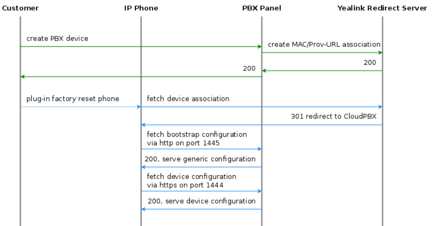
Figure 128: Initially bootstrap a Yealink phone
