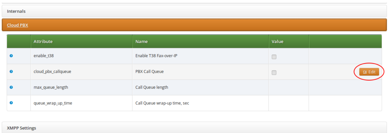
Figure 102: Call Queue Configuration
