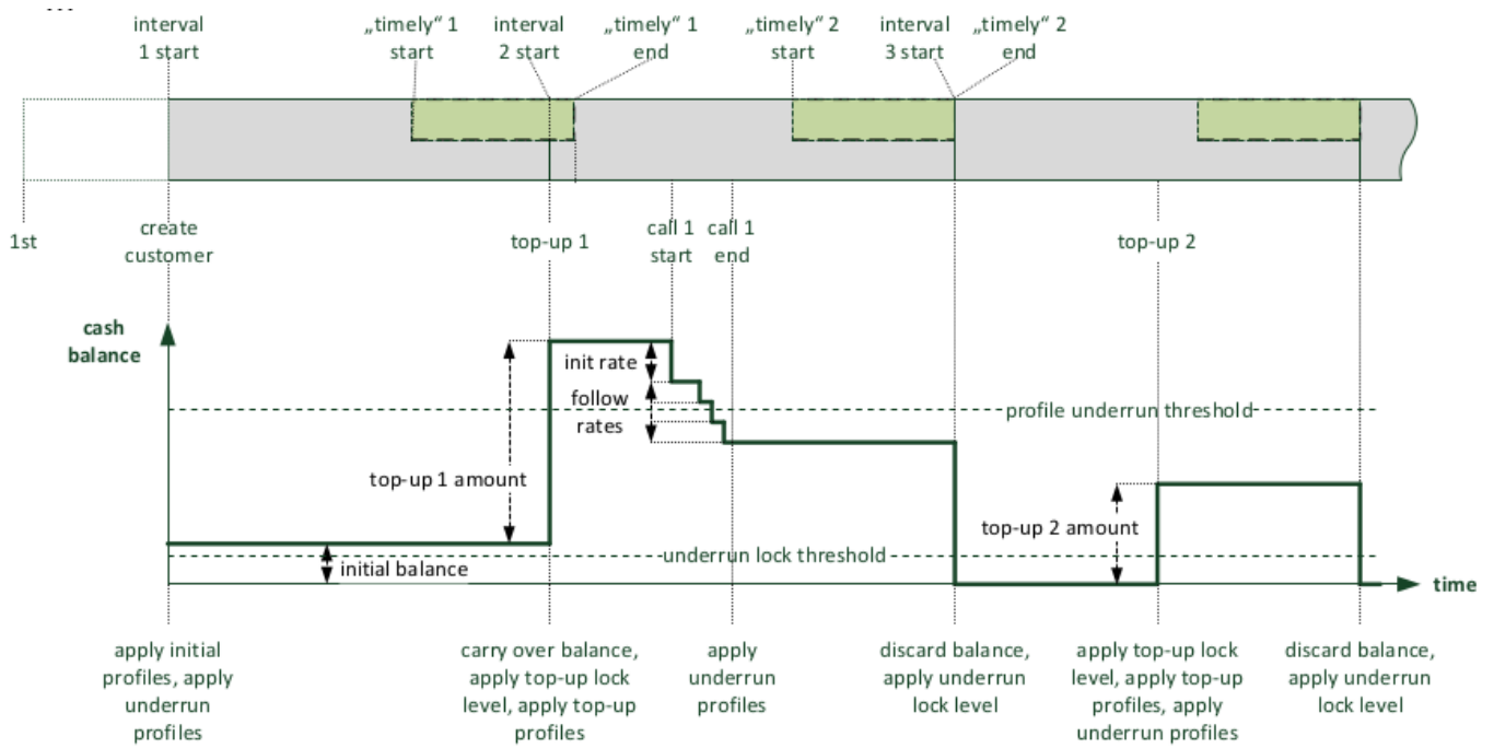
Figure 49: Example: Top-up Interval and Timely Carry-over
