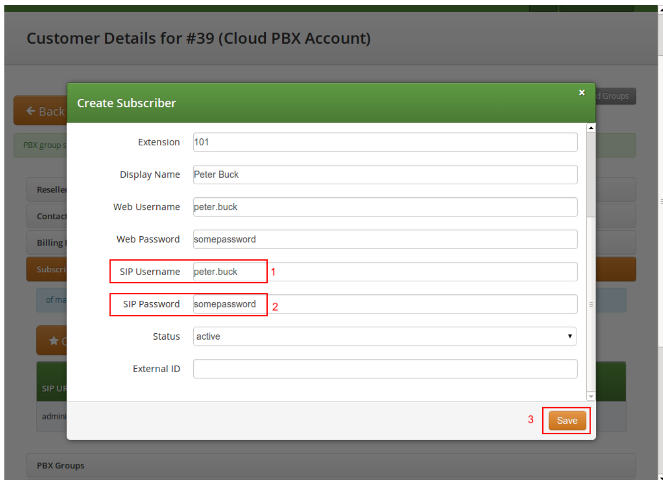
Figure 83: Finish PBX Subscriber Creation Part 2
