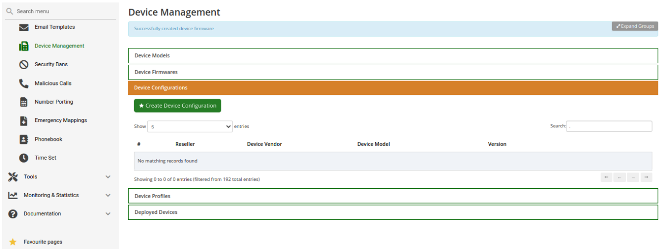
Figure 193. Device Configuration
