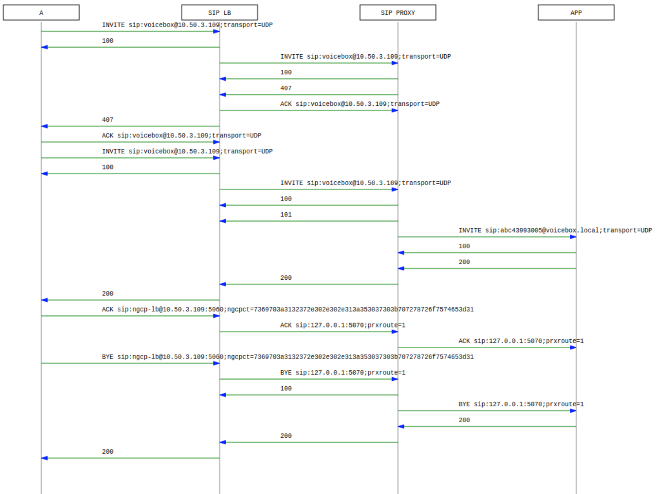
Figure 229. Voicebox Call-Flow
