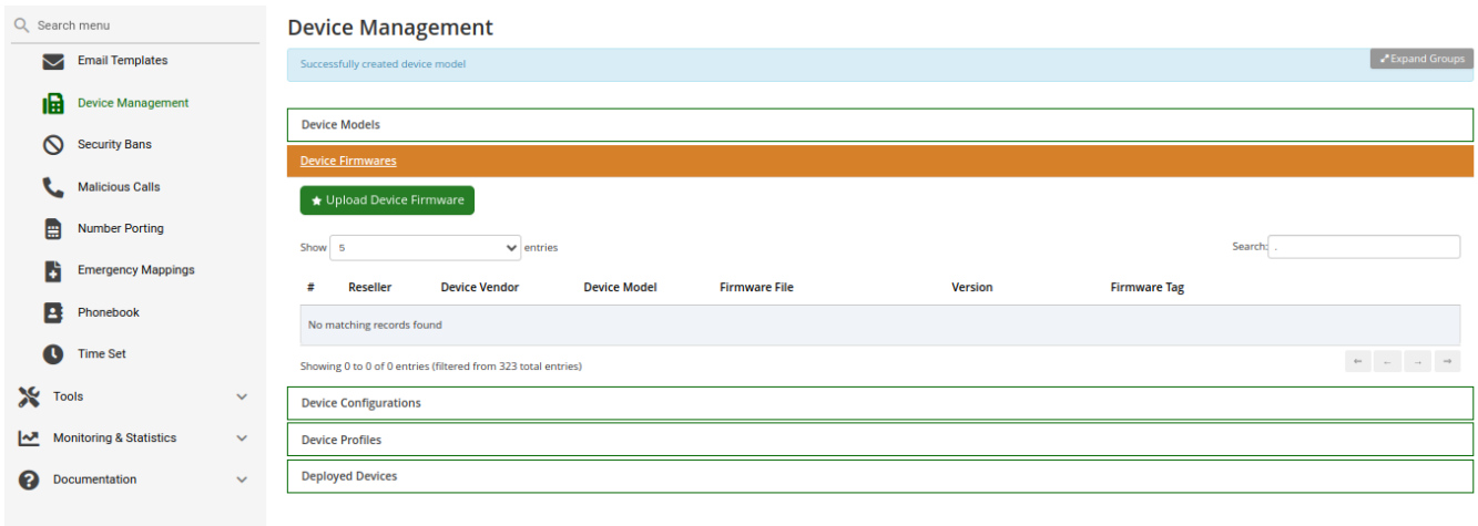
Figure 191. Device Firmware
