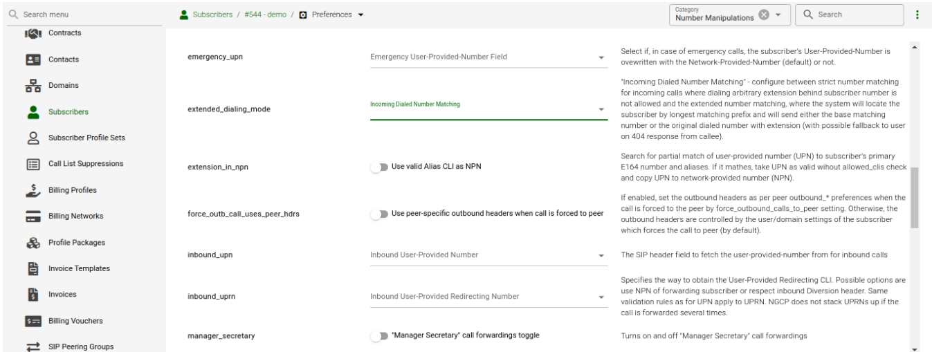
Figure 92. Subscriber Preferences - extended_dialing_mode
