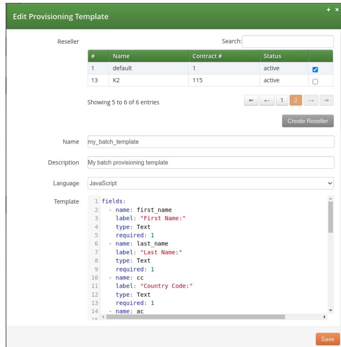
Figure 130. Create Provisioning Template.
