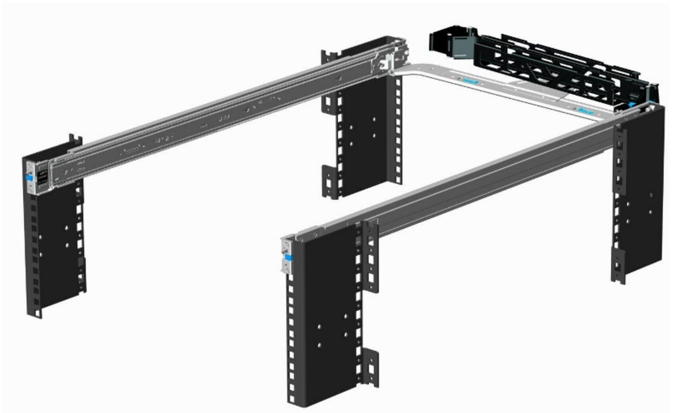
Figure 8. Rack-mounted Rails
