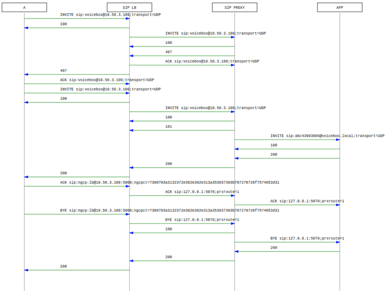
Figure 84. Voicebox Call-Flow
