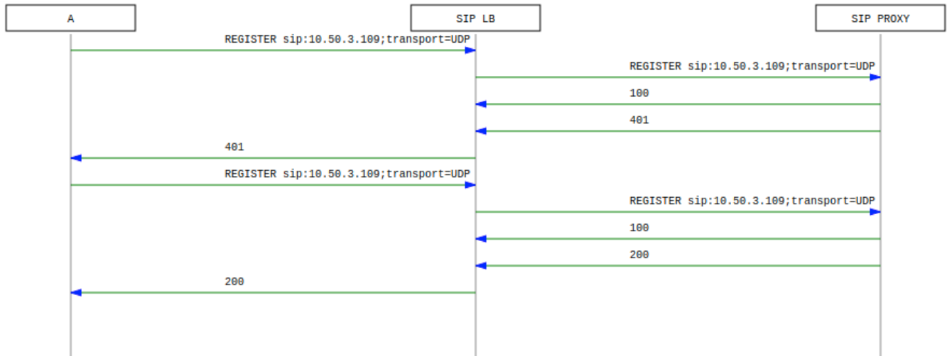
Figure 179. Registration Call-Flow
